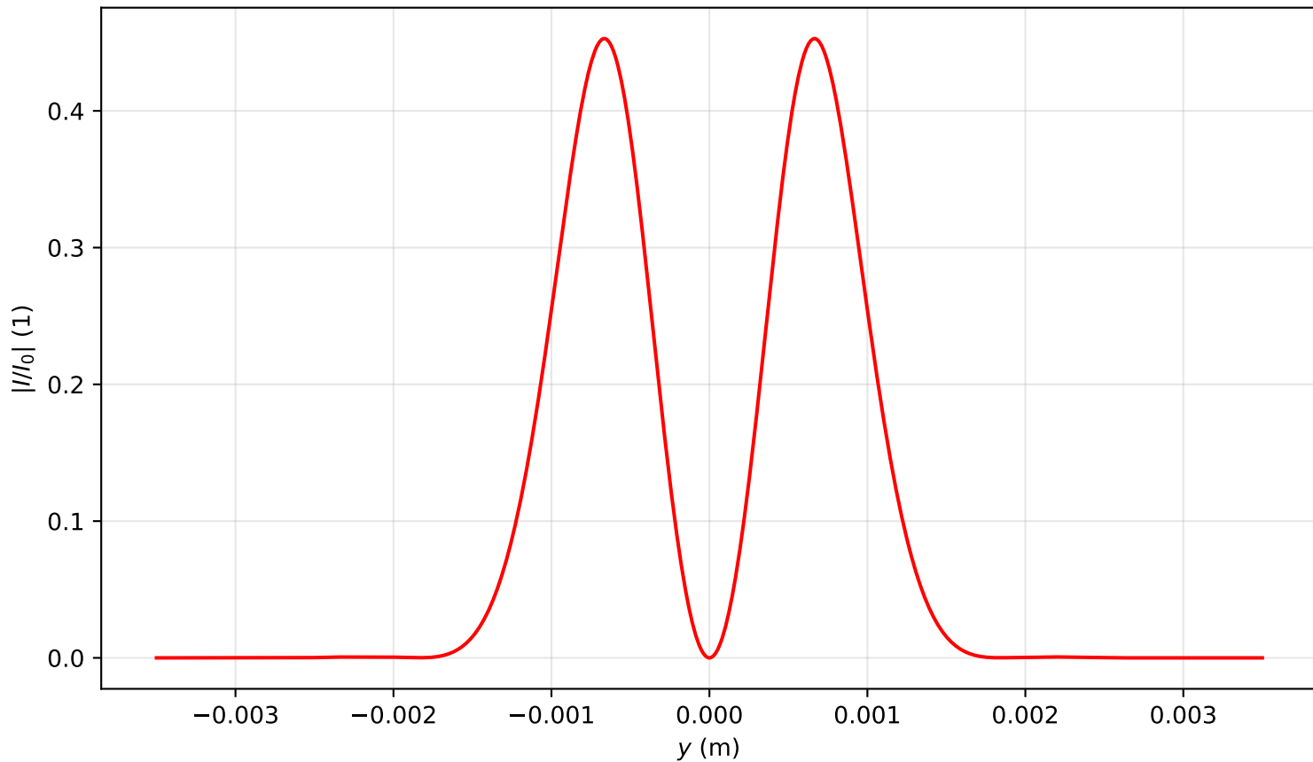
Intensity profile I(x=0, y, z=1.911)/I_0 , P_{in}=2.0P_{cr} , artificial time
